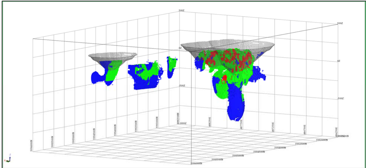
Figure 14.36: Oblique view to the Southeast of the Minago Project mineral resource categorization with pit shell in grey (Category: Blue - Inferred, Green – Indicated, Red – Measured)
