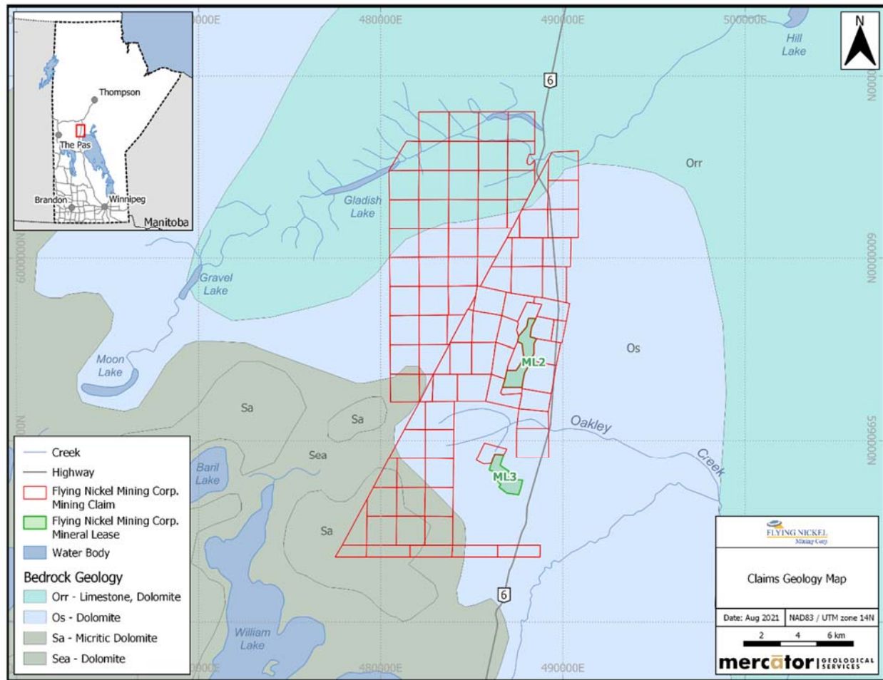
Figure 7.2: Minago Nickel Project surface geology map
