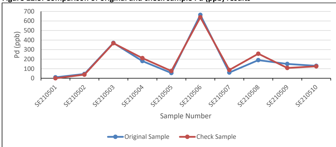
Figure 12.3: Comparison of original and check sample Pd (ppb) results
